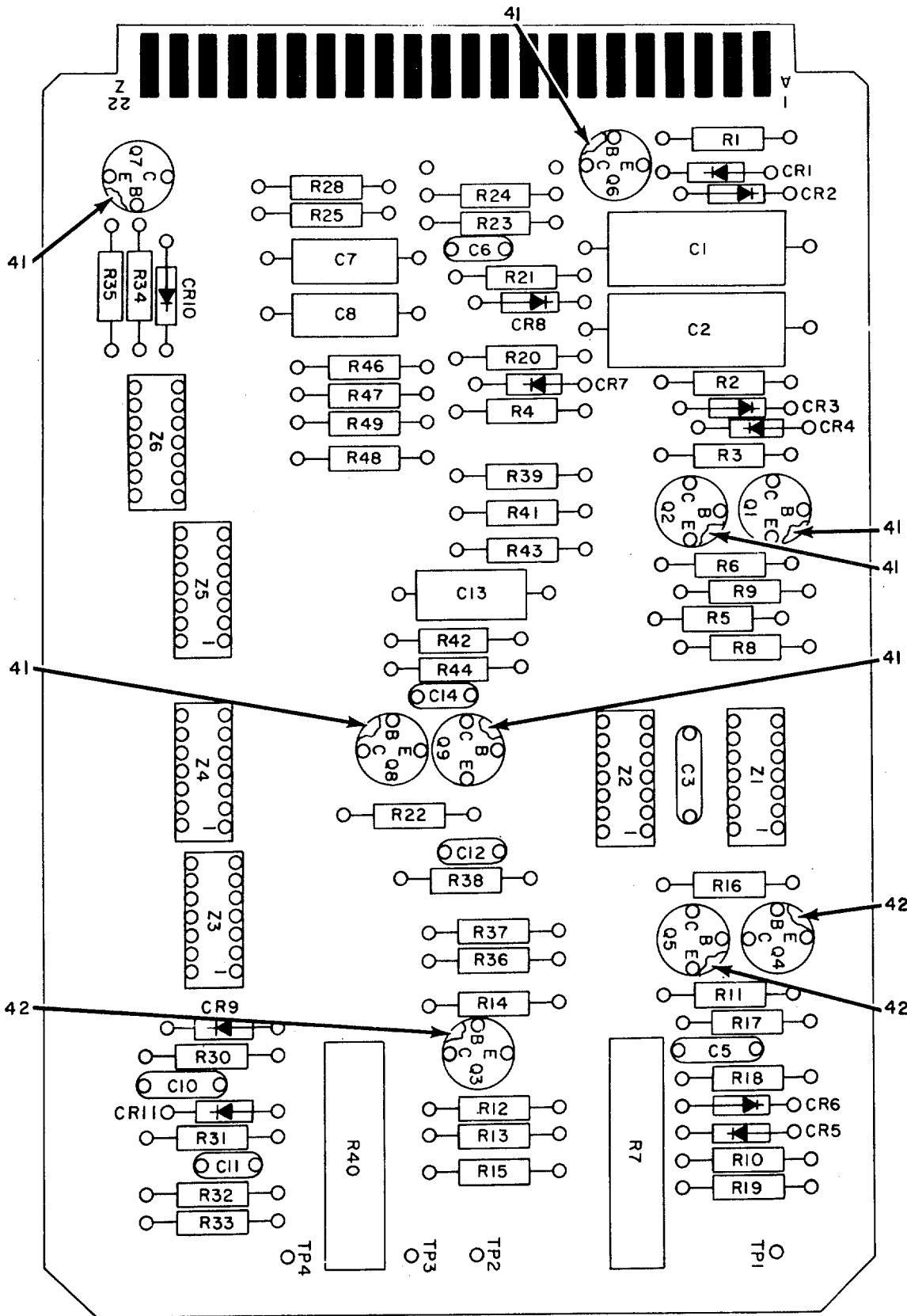
Figure 8. Component Board Assembly SMD633072 3A3A3 (Sheet 1 of 2).
