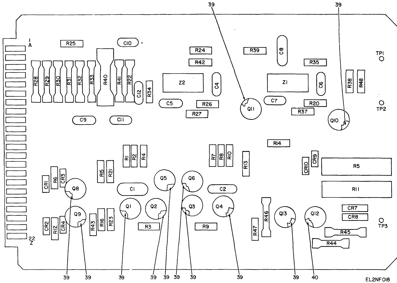
Figure 12. Component Board Assembly SMD633076 3A3A7 (Sheet 1 of 2).
