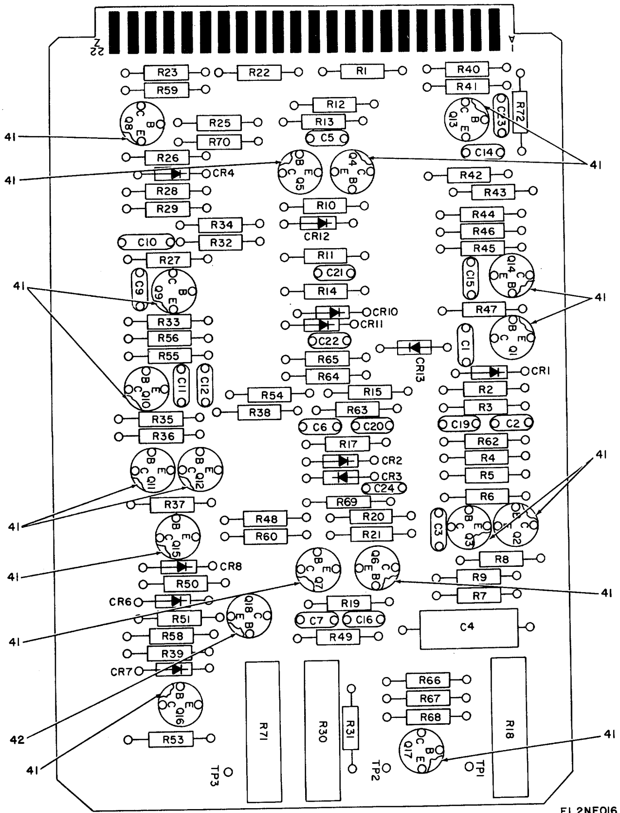
Figure 11. Component Board Assembly SMD633075 3A3A6 (Sheet 1 of 2)
