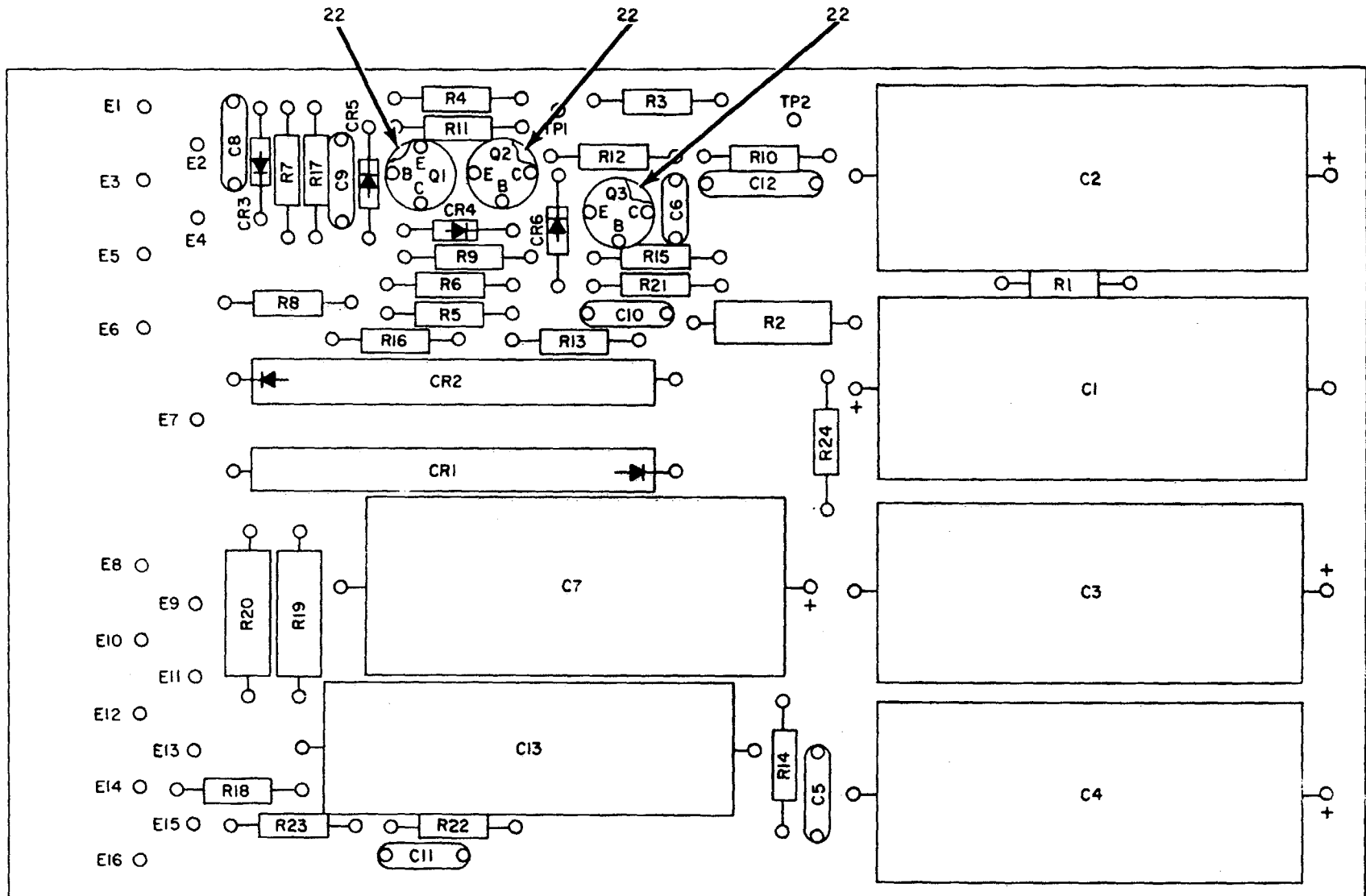
Figure 14. Component Board Assembly SMD633078 3AA1 (Sheet 1 of 2).
