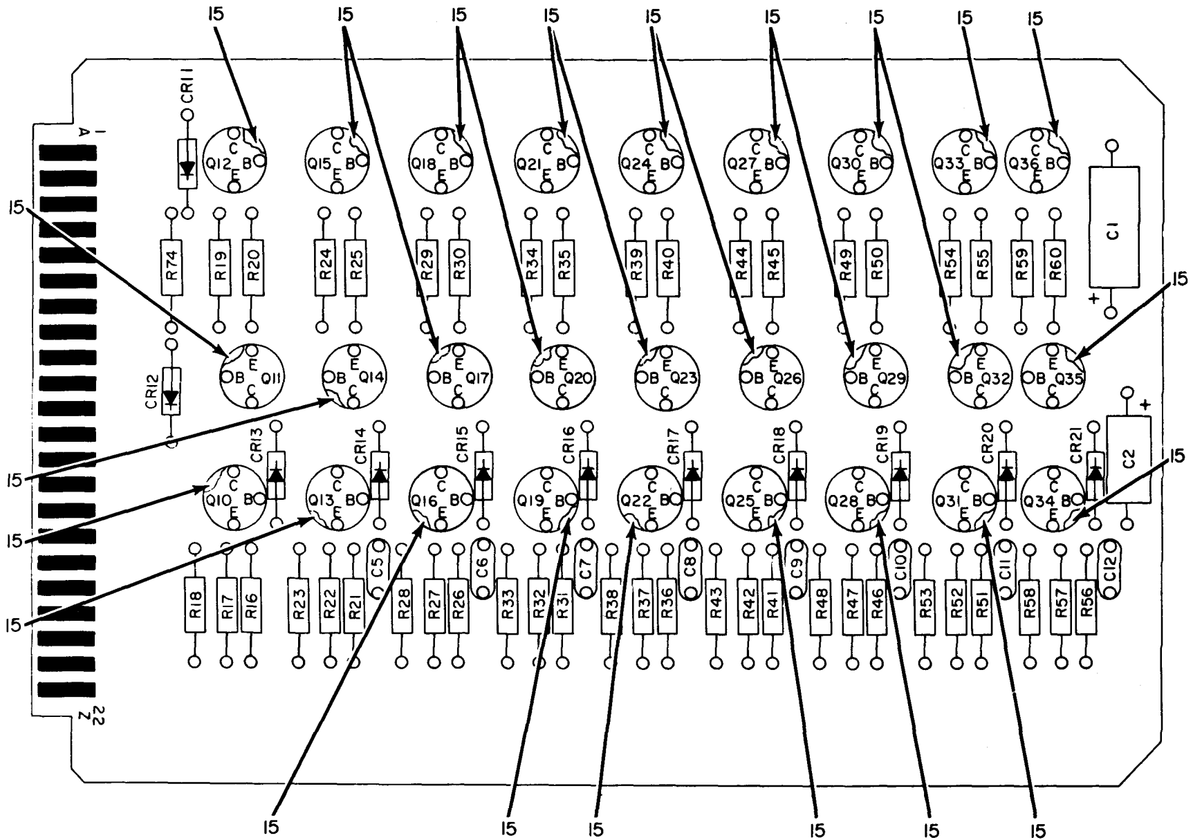
Figure 9. Component Board Assembly SMD633073 3A3A4 (Sheet 1 of 2).
