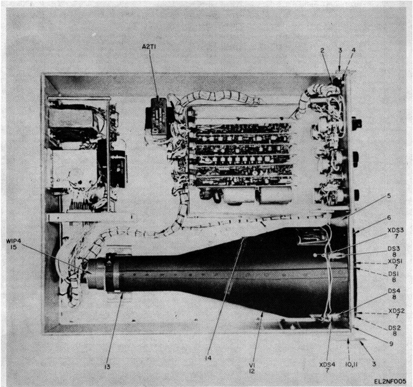
Figure 4. Chassis Assembly, Scope SMD32993 3A2.
