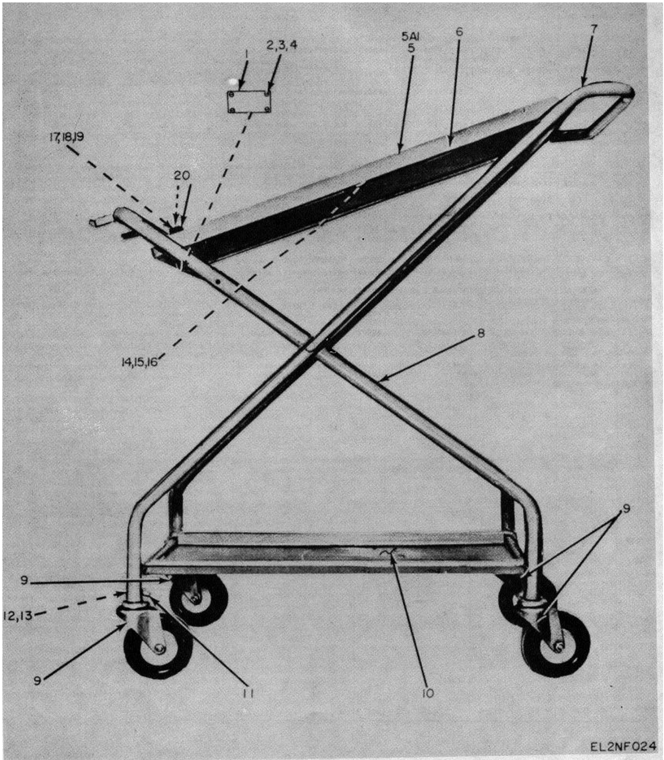
Figure 16. Dolly, Test Equipment V-434/GGM-15(V) (Used On V2 Only) .
