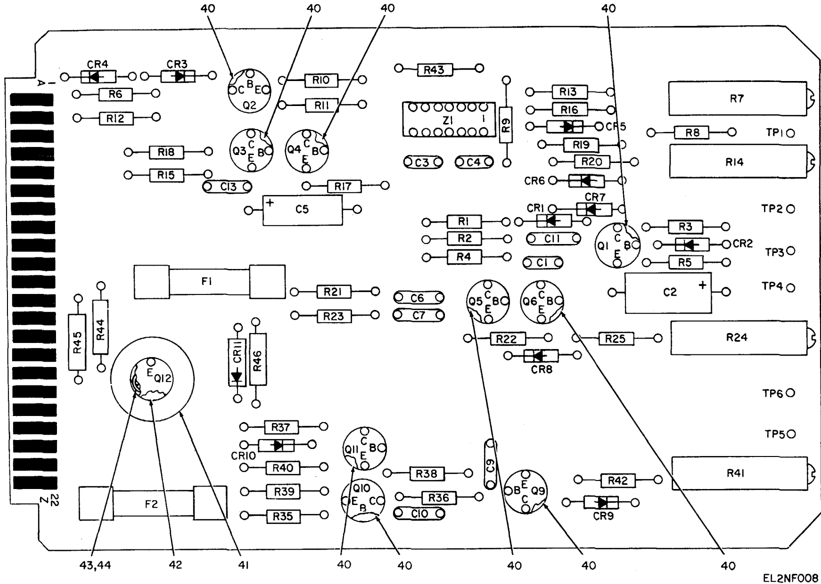
Figure 7. Component Board Assembly SMD633071 3A3A2 (Sheet 1 of 2).
