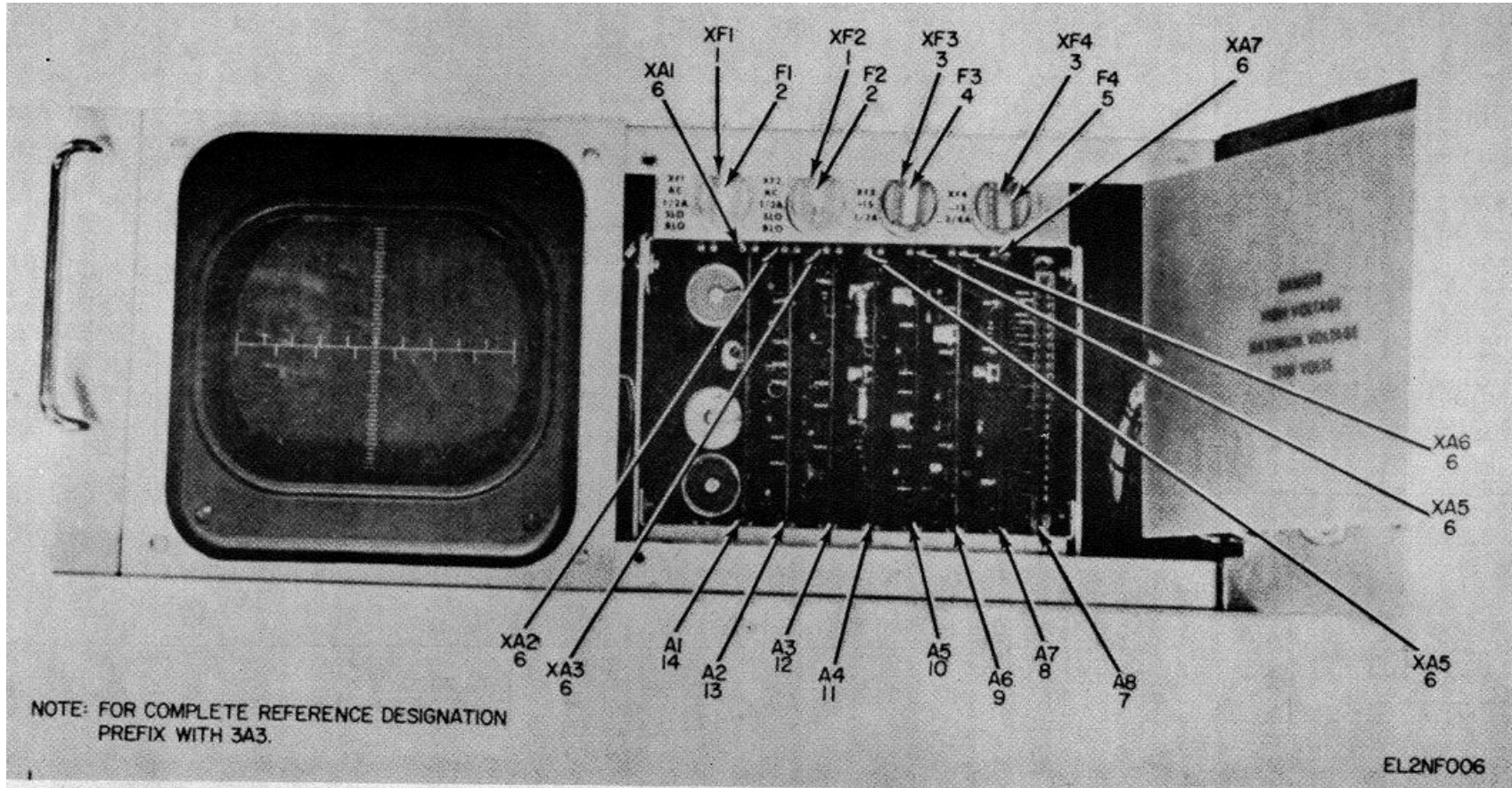
Figure 5. Cage Assembly SMD633004 3A3.
