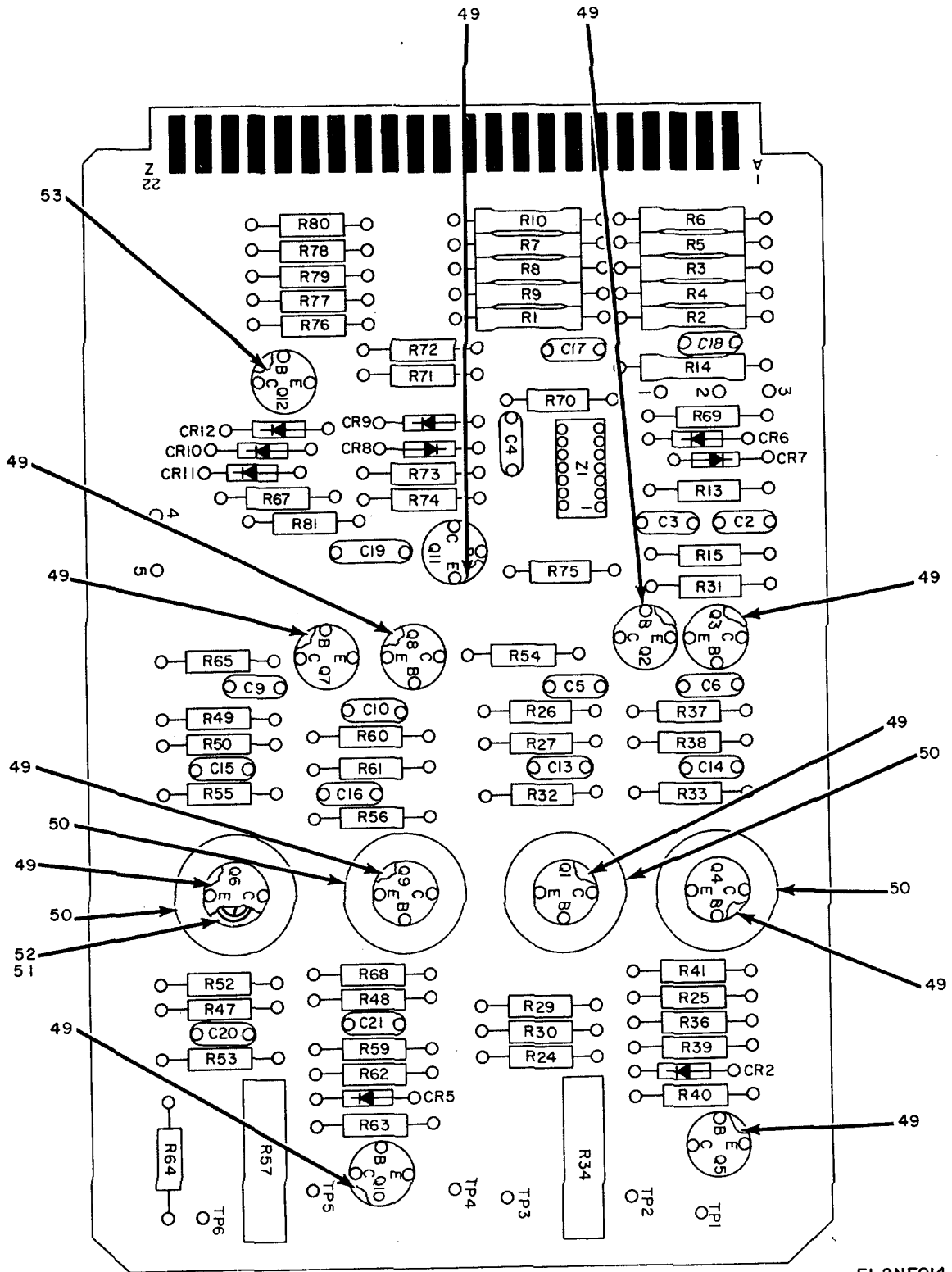
Figure 10. Component Board Assembly SMD633074 3A3A5 (Sheet 1 of 2).
